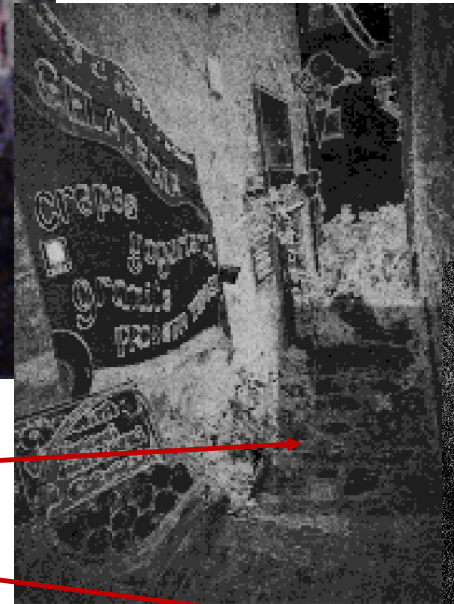
DCT Map
